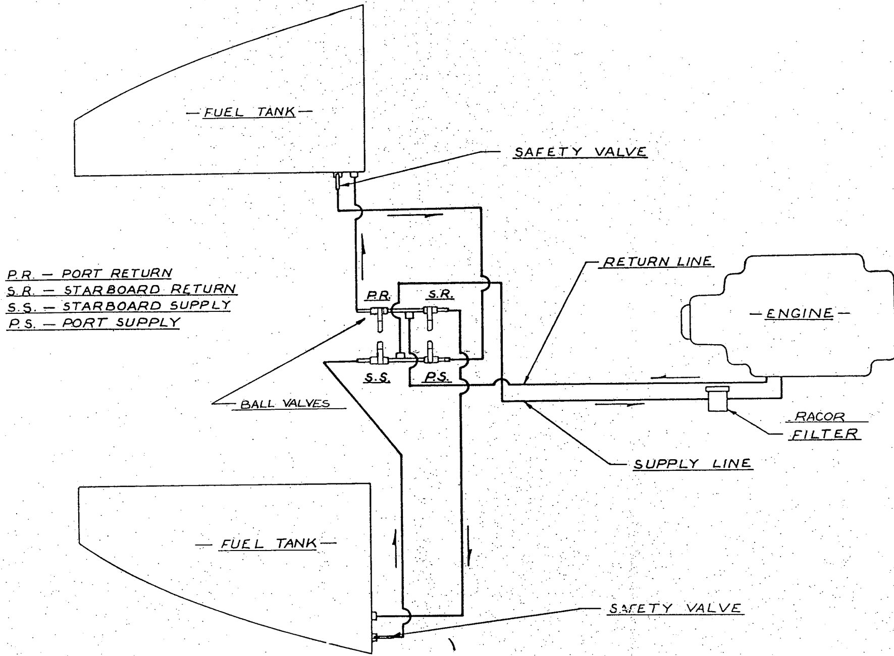
— FUEL SUPPLY & RETURN SYSTEM —
