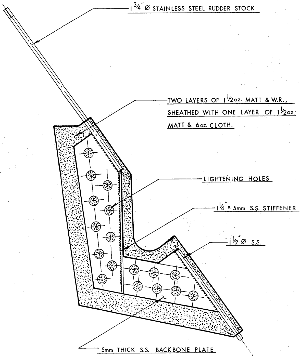
MASON 44 RUDDER CONSTRUCTION, NOTE ABUNDANCE OF STAINLESS STEEL REINFORCEMENT WITHIN THE RUDDER STRUCTURE.
