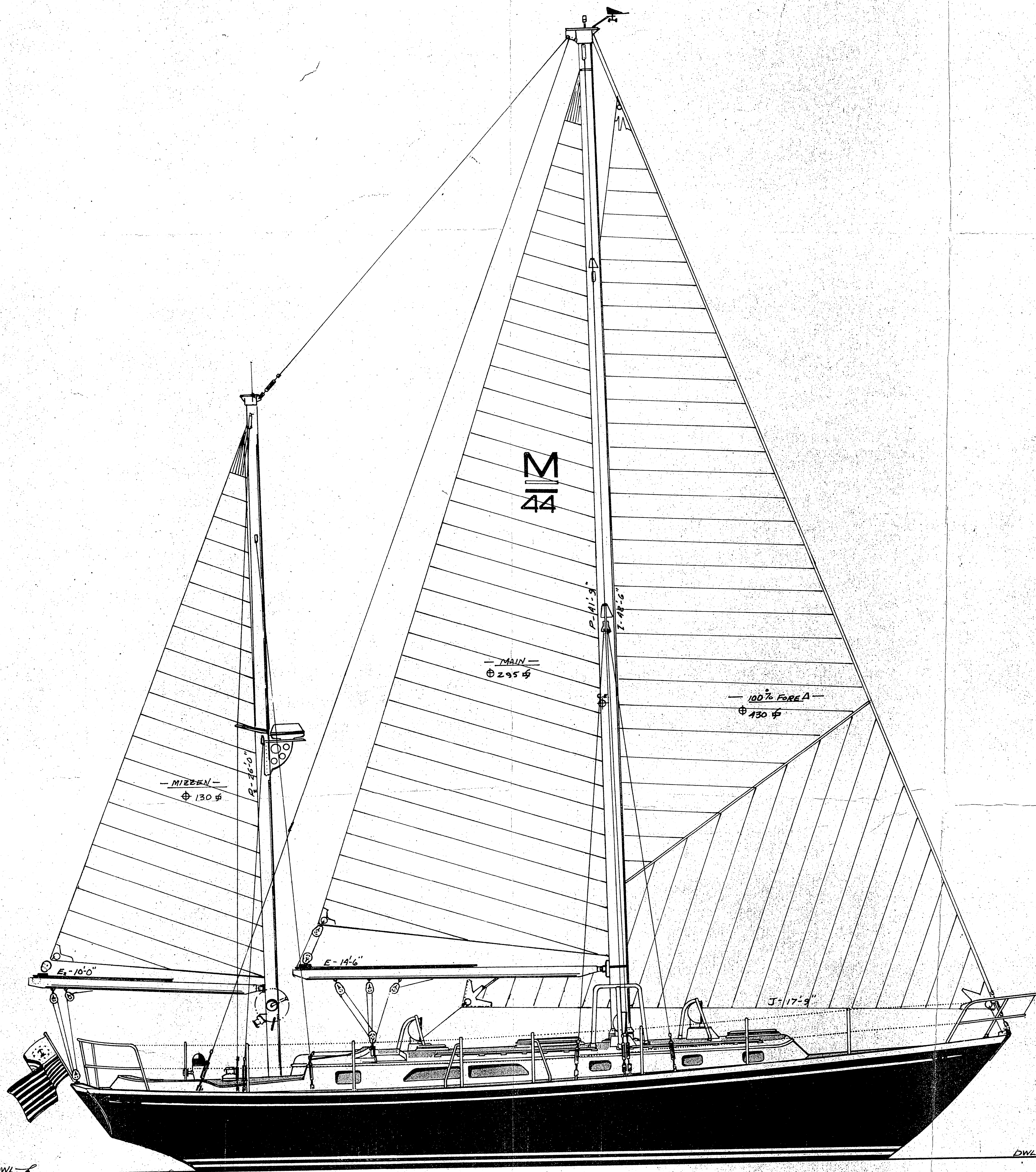
—SAIL PLAN—
